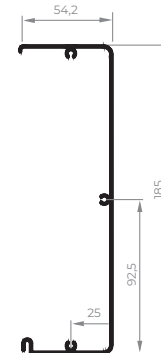
EXL-032 Tampa externa porta integrada 1,494 kg/m
