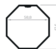
EXL-610 Tubo octogonal 60 mm 0,766 kg/m
