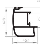
EXL-350 Montante bi-tubular central externo 0,714 Kg/m
