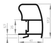
EXL-504 Montante bi-tubular central interno 0,790 Kg/m
