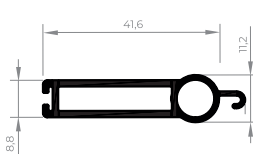
EXL-055 Terminal persiana 48 mm 0,352 Kg/m
