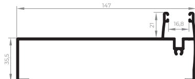
EXL-337 Complemento lateral persiana 3 planos 1,163 Kg/m
