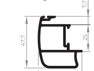
EXL-350 Montante bi-tubular central externo 0,714 Kg/m
