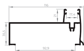
EXL-513 Complemento lateral persiana 1,015 Kg/m
