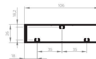
EXL-013 Coluna 3 planos 1,418 Kg/m
