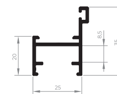
EXL-079 Marco perimetral maxim-ar 0,315 Kg/m
